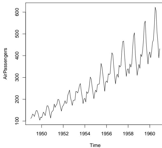
Figure 8.1: A Time Series of AirPassengers
